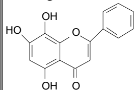
Norwogonin [4443-09-0]
